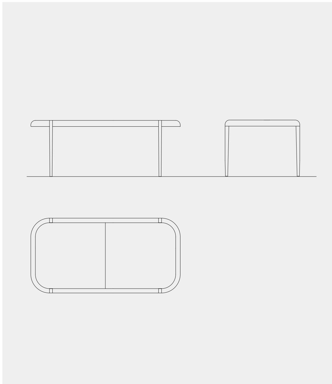
LOLA TABLE - R818 - 200 X 100 X 75CM
