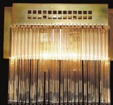
Wall light III. ↑25 cm ↔29 cm |→13 cm 2 x 60 W E14 0.7 Kg
