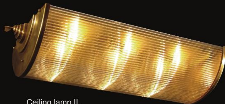
Ceiling lamp II. ↕ 20 cm ↔ 80 cm ↳ 40 cm 8 x 60 W E14 4 Kg
